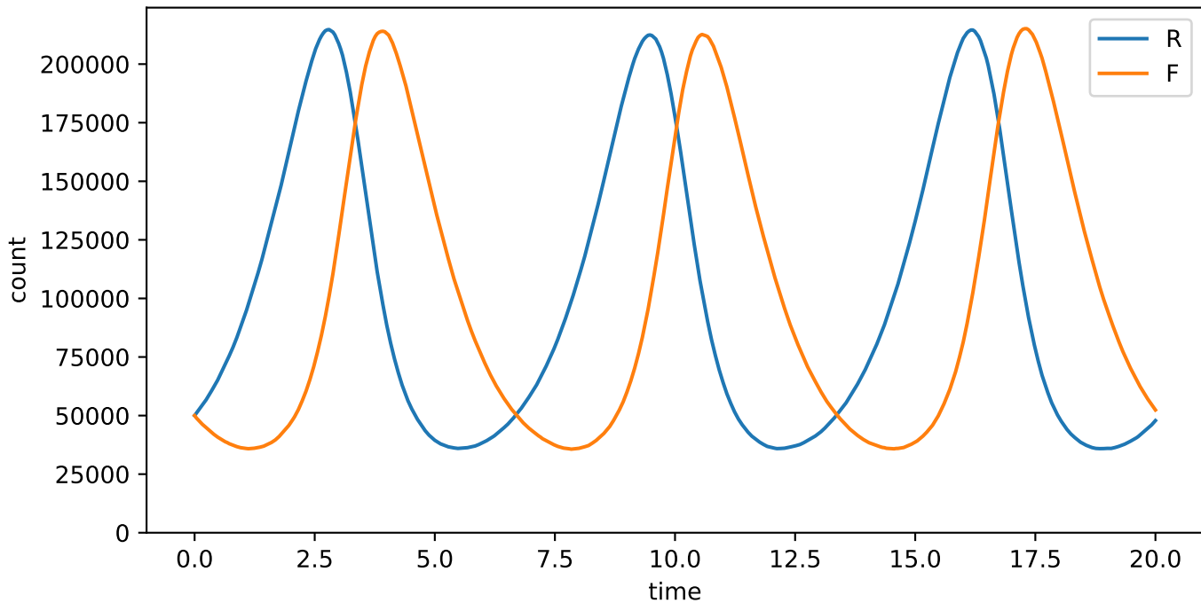
Lotka Volterra: rebop, n=10^5
